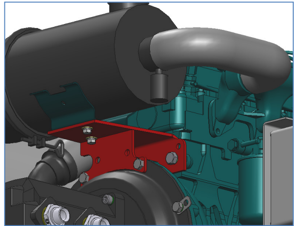
Figure 2 – New Bracket PP-41233
